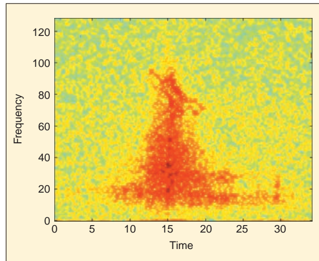
▲ 8. STFT of a seismic signal due to a moving vehicle.
