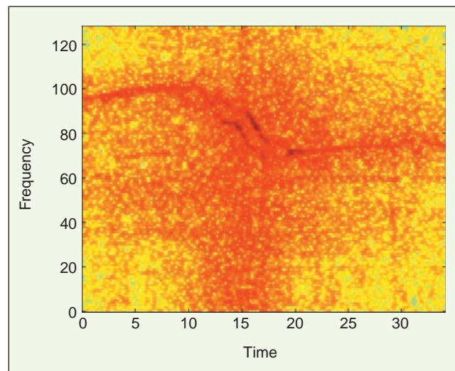
▲ 9. STFT of an acoustic signal due to a moving vehicle.
