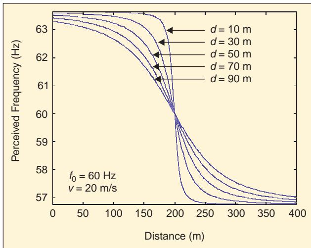
▲ 7. Plots of perceived frequency for acoustic signals as a function of source position for different values of d .
