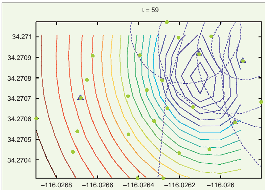
▲ 3. Illustration of energy-based collaborative target localization using real seismic (noisy) data. Dots indicate node locations. Triangles indicate the four nodes being used in the position calculation. Dashed circles indicate loci of possible target locations based on the six ratios of sensor readings. Three different points can be identified at which three of the six circles intersect, suggesting possible target locations. Solid lines represent constant-value contours of the cost function. The center of the contour plots indicates estimated target location and is inside the region bounded by the three intersection points of circles.
