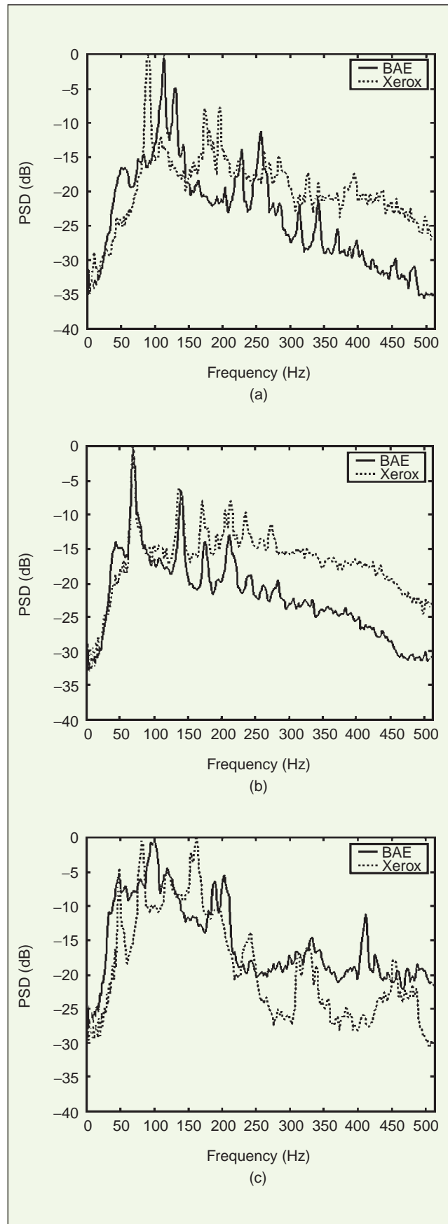
▲ 5. (a) Acoustic PSD of a wheeled vehicle (08020830 DW). (b) Acoustic PSD of a tracked vehicle (08030800 AAV). (c) Acoustic PSD of a wheeled vehicle (08040820 LAV).
