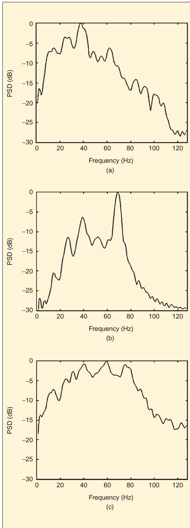
▲ 4. (a) Seismic PSD of a wheeled vehicle (08020830 DW). (b) Seismic PSD of a tracked vehicle (08030800 AAV). (c) Seismic PSD of a wheeled vehicle (08040820 LAV).
