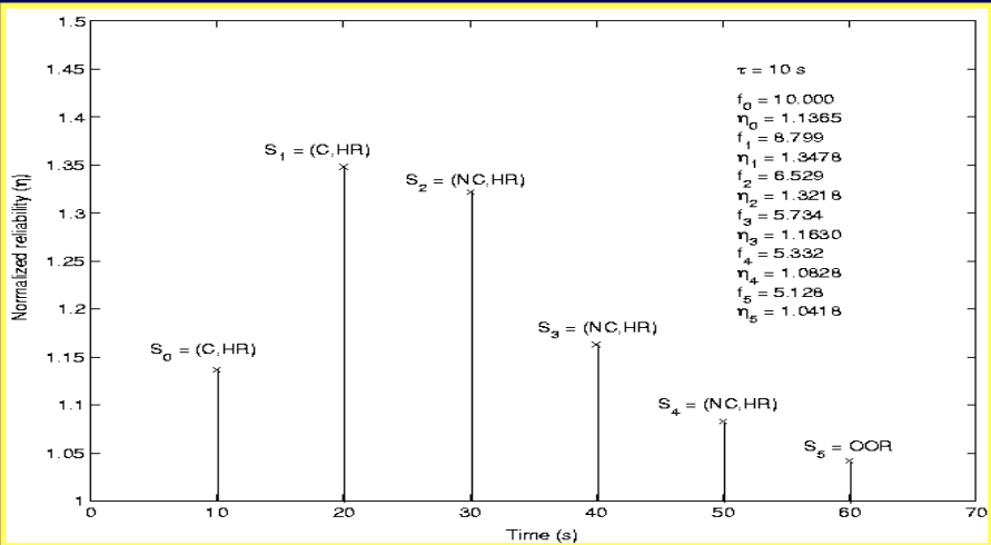
S_0 = (C,HR)
