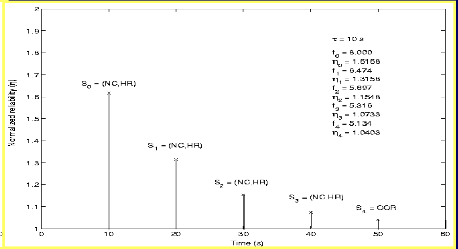
S_0 = (NC,HR)
