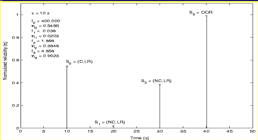
S_0 = (C,LR)
