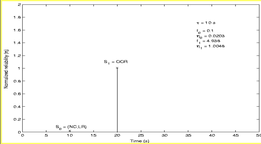
S_0 = (NC,LR)
